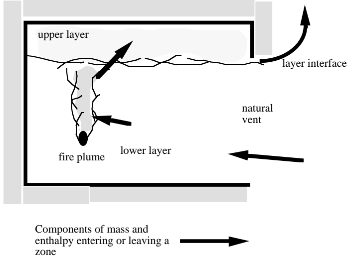
Figure 2: Two Layer Zone Model Setup
