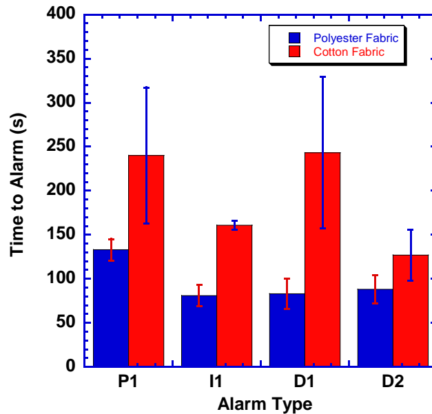
Figure 7. Average alarm time for flaming, low density foam, living room fires. Comparison between the polyester (configuration 5) and cotton (configuration 7) fabrics. Error bars are one standard deviation.
