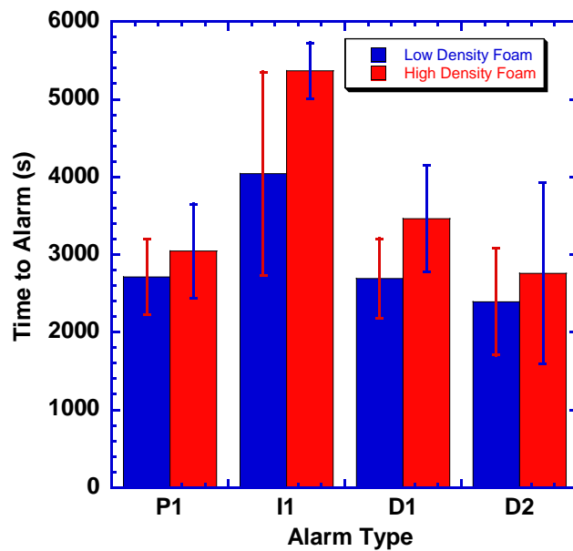
Figure 5. Average alarm time for living room smoldering fire, cotton fabric tests. Comparison between foam density, low (configuration 3) and high (configuration 4). Error bars are one standard deviation.
