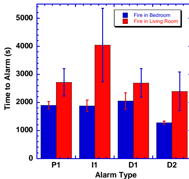
Figure 4. Average alarm time for smoldering, low density foam, cotton fabric tests. Comparison between the fire located in bedroom (configuration 1) versus the living room (configuration 3). Error bars are one standard deviation.
