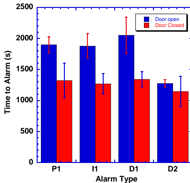
Figure 3. Average alarm time for smoldering, low density foam, cotton fabric tests. Comparison between the bedroom fire with the door opened (configuration 1) or closed (configuration 2). Error bars are one standard deviation.
