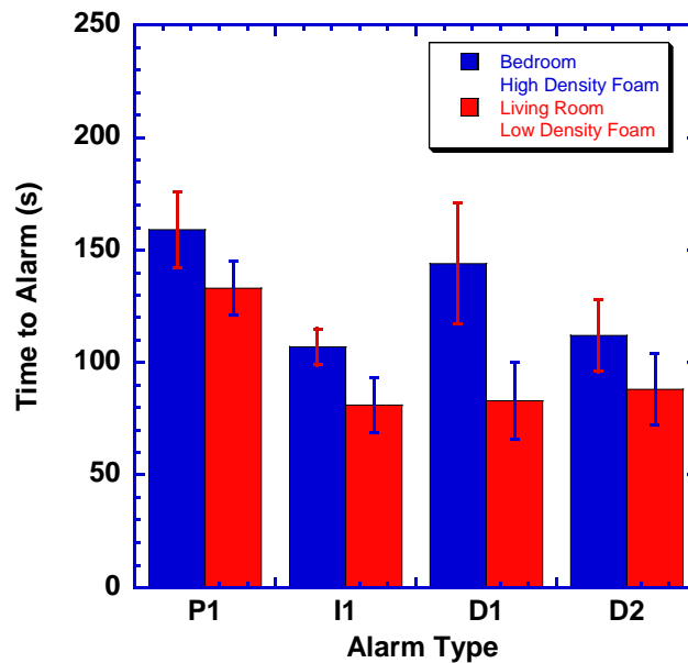
Figure 9. Average alarm time for flaming, polyester fabric fires. Comparison between configuration 8 (bedroom, high density foam fire) and configuration 5 (living room, low density foam fire). Error bars are one standard deviation.
