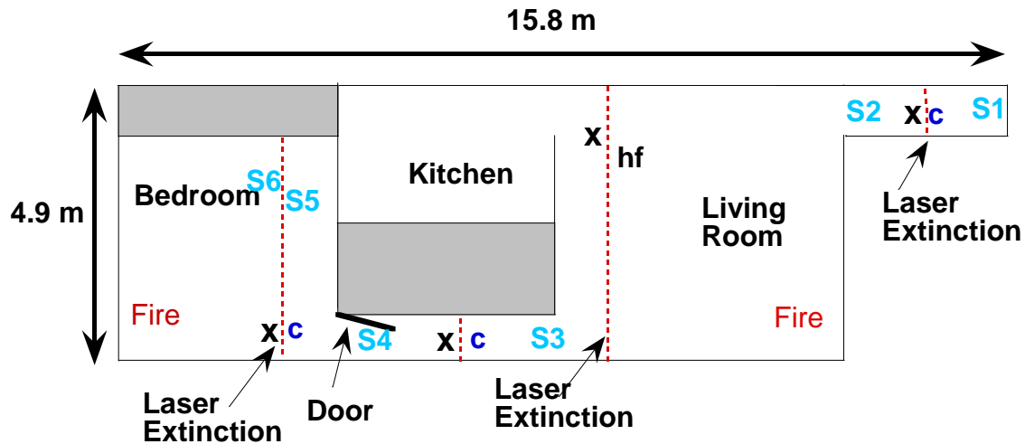
Figure 1. Schematic of the test structure. An X indicates a thermocouple tree. hf shows the location of the total heat flux gage, which was 1.5 m above the floor and pointing toward the fire source. S1...S6 indicate alarm set locations. c indicates gas sampling locations located 1.5 m above the floor. Hydrogen cyanide was sampled at the gas sampling location in the hallway between the bedroom and living room. The dashed lines represent laser beam paths for extinction measurements located 1.5 m above the floor.
