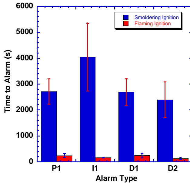
Figure 6. Average alarm time for living room, low density foam, cotton fabric tests. Comparison between smoldering (configuration 3) and flaming (configuration 7) fires. Error bars are one standard deviation.
