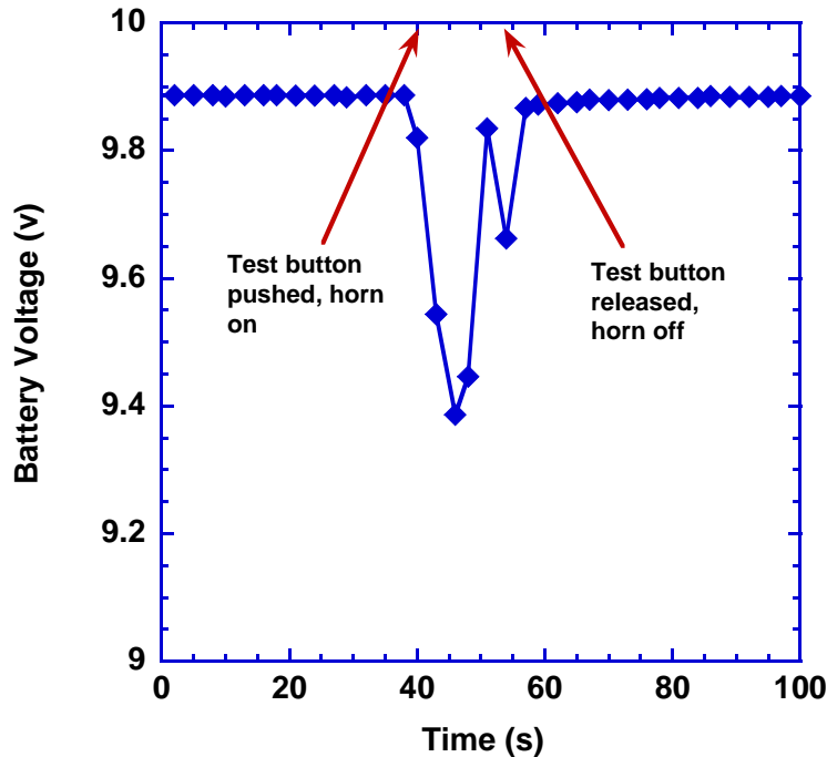
Figure 2. A representative plot of alarm battery voltage signal when the test button was depressed and released.
