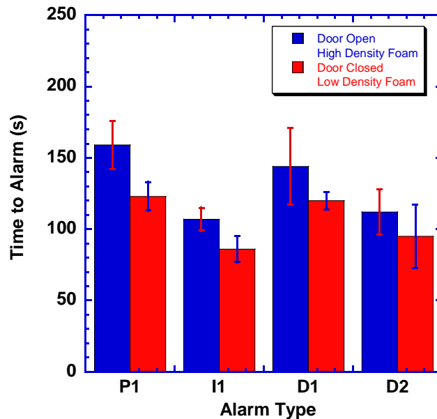
Figure 8. Average alarm time for flaming, polyester fabric, bedroom fires. Comparison between configuration 8 (door open, high density foam) and configuration 6 (door closed, low density foam). Error bars are one standard deviation.
